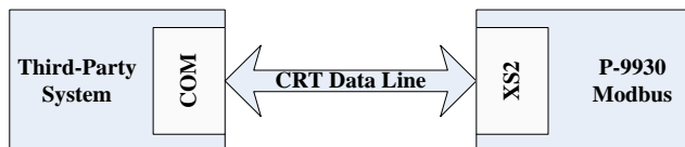
Fig. 2 RS232 connection
