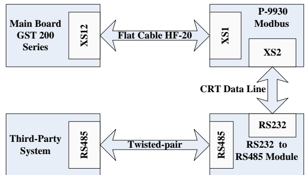
Fig. 3 RS485 Connection
